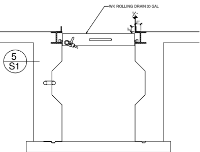
ROLLING DRAIN
