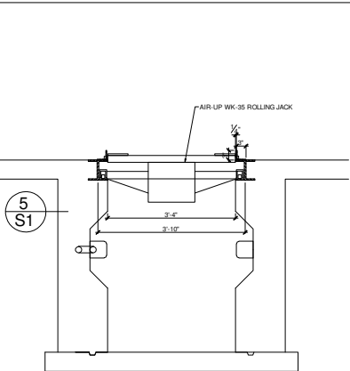
PIT JACK
